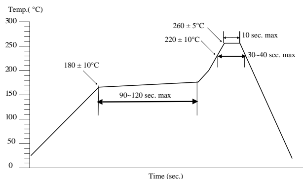
Reflow profile
